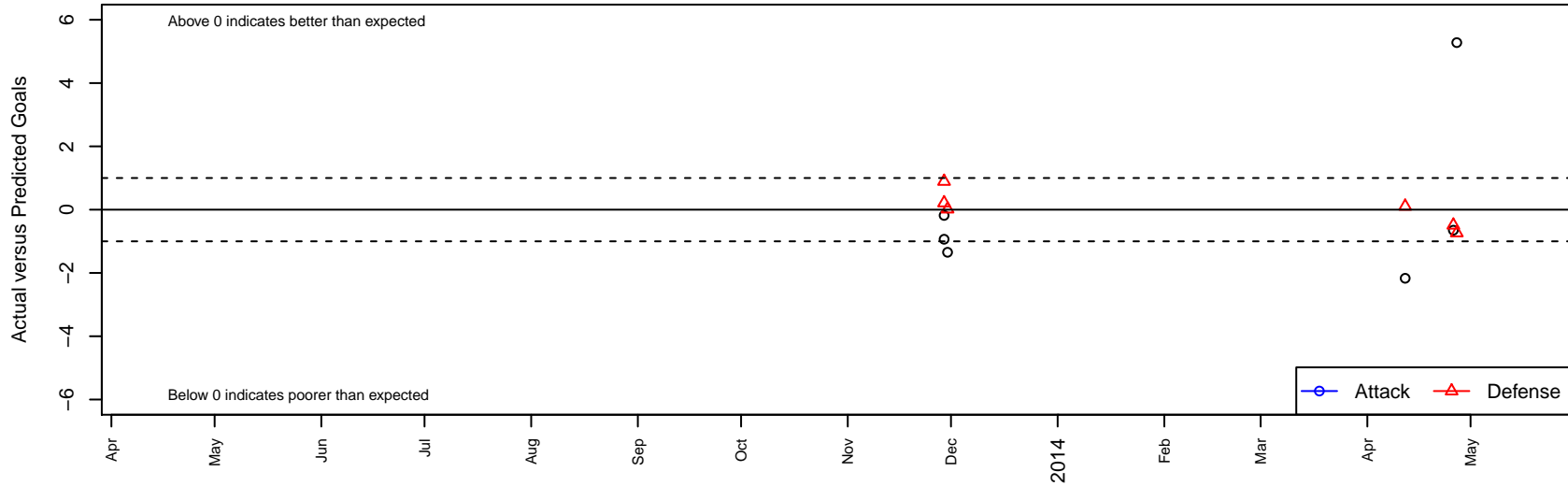
CYSL Nado Premier B99 Dots are actual minus expected GF (blue circles) and GA (red triangles). Blue line is smoothed change in attack strength. Red is smoothed change in defense strength.
